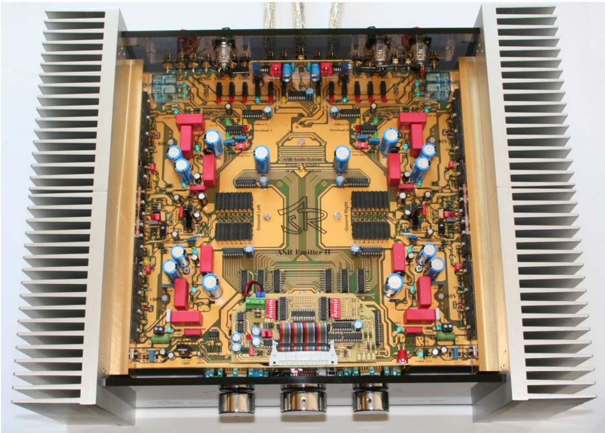
Emitter II Exclusive with gold plated pcb boards from 2007 on
