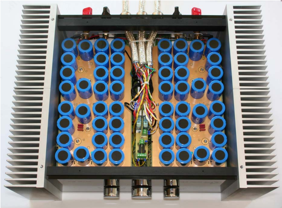
Emitter II Exclusive double sides Elko boards from 2007 on
